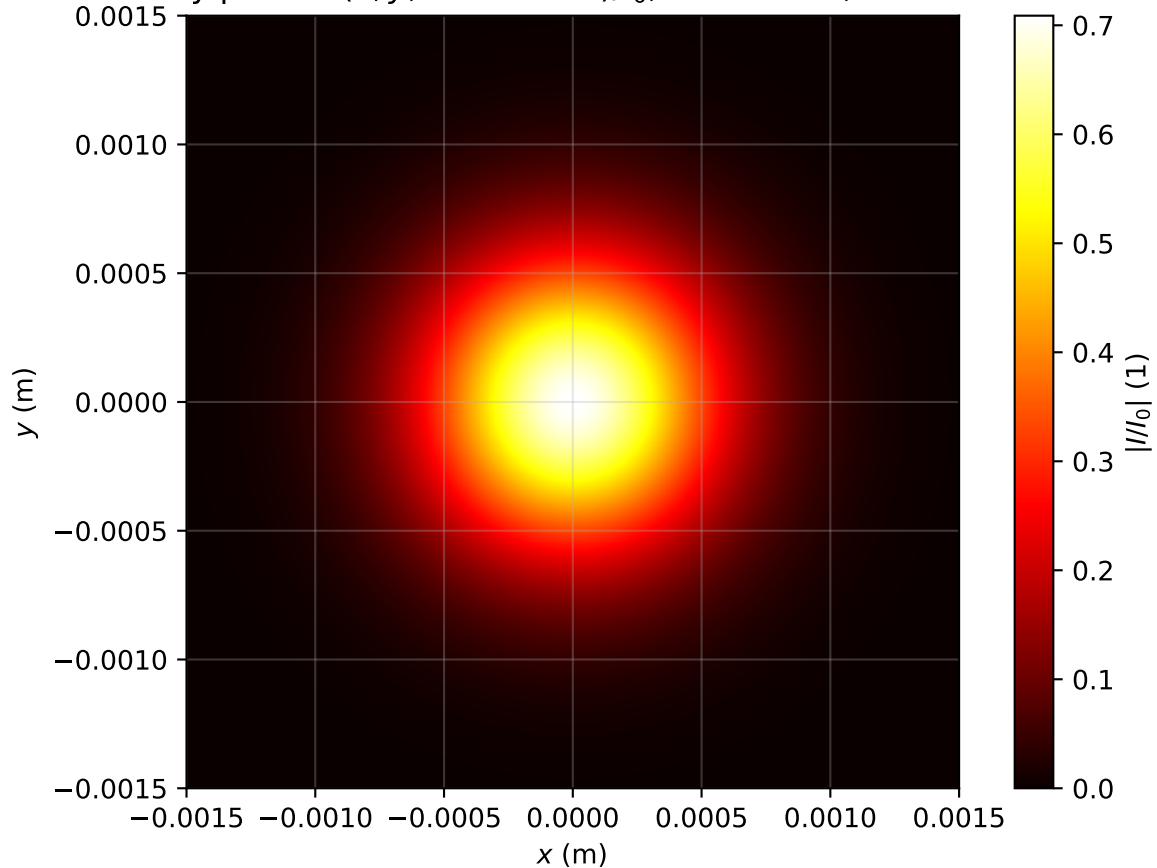
Intensity profile I(x, y, z = 1.592m)/I_0 , Pin=0.2Pcr, artificial time
